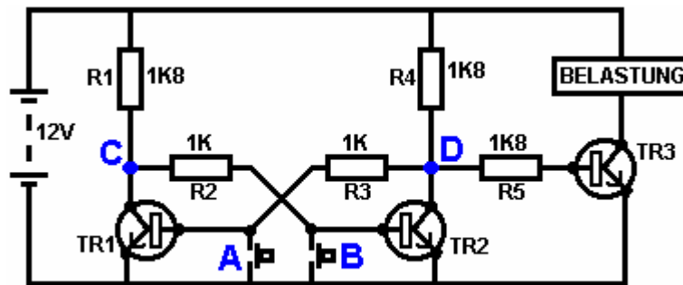
Bistabilen Multivibrator
